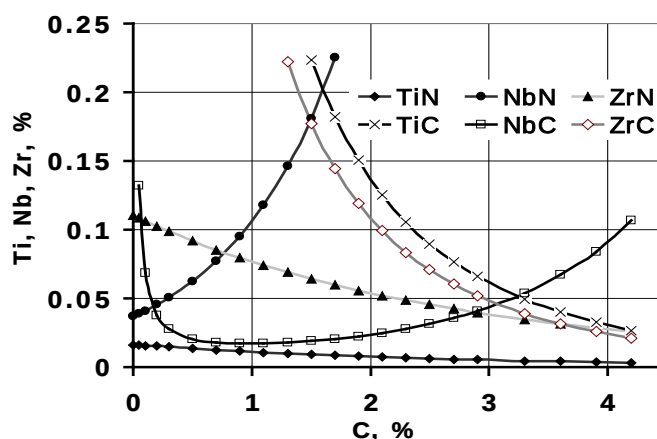
Fig. 1. The dependence of equilibrium with the nitride or carbide content of Ti, Nb, Zr and carbon in Fe-base melt
